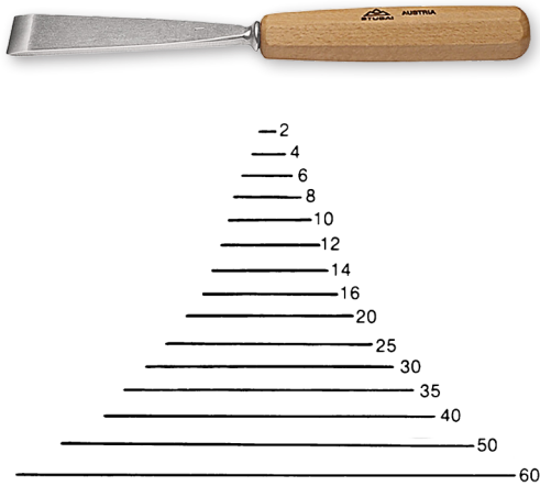
No. 5501 Straight Chisel
